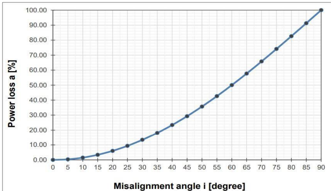
Relation between solar panel misalignment and direct power loss:
