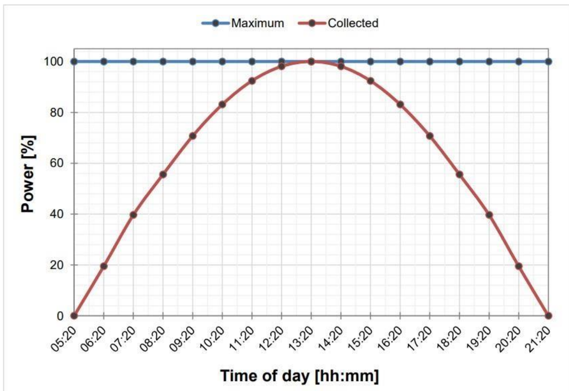
Approximation of power output (red line) compared to maximum output (blue line) for a fix mounted solar module:
