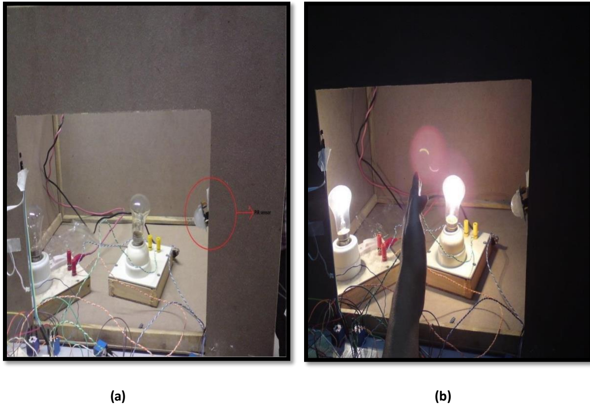
Figure 5.7 Practical implementation of control of lighting system. (a) No human body, (b) with human body.
