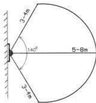
Figure 2.4: PIR sensor range and its lens angle
